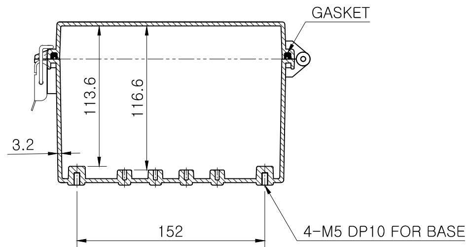
SECTION B-B
